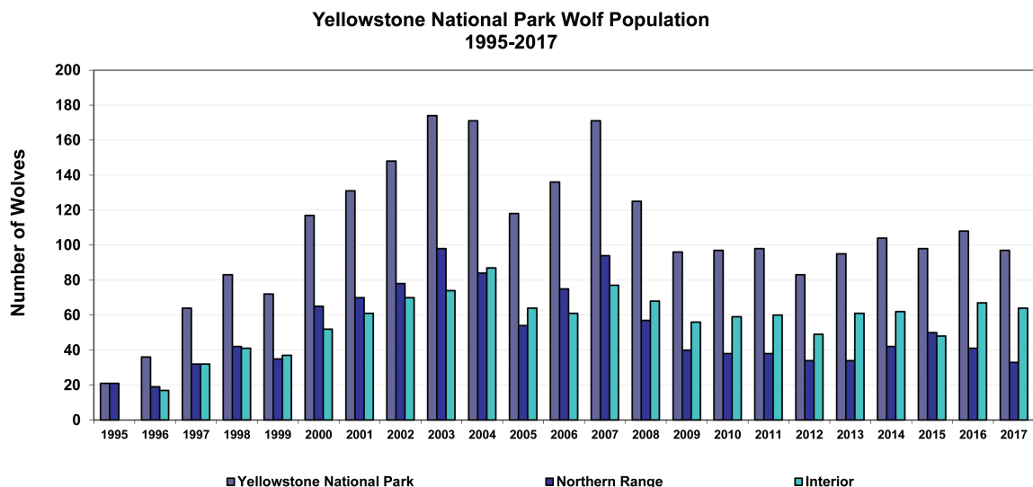
Fig. 1.—Census of wolves ( Canis lupus ) in Yellowstone National Park, 1995–2017, including a breakdown for the Northern Range and the interior portions of the park. Courtesy of Yellowstone National Park.
