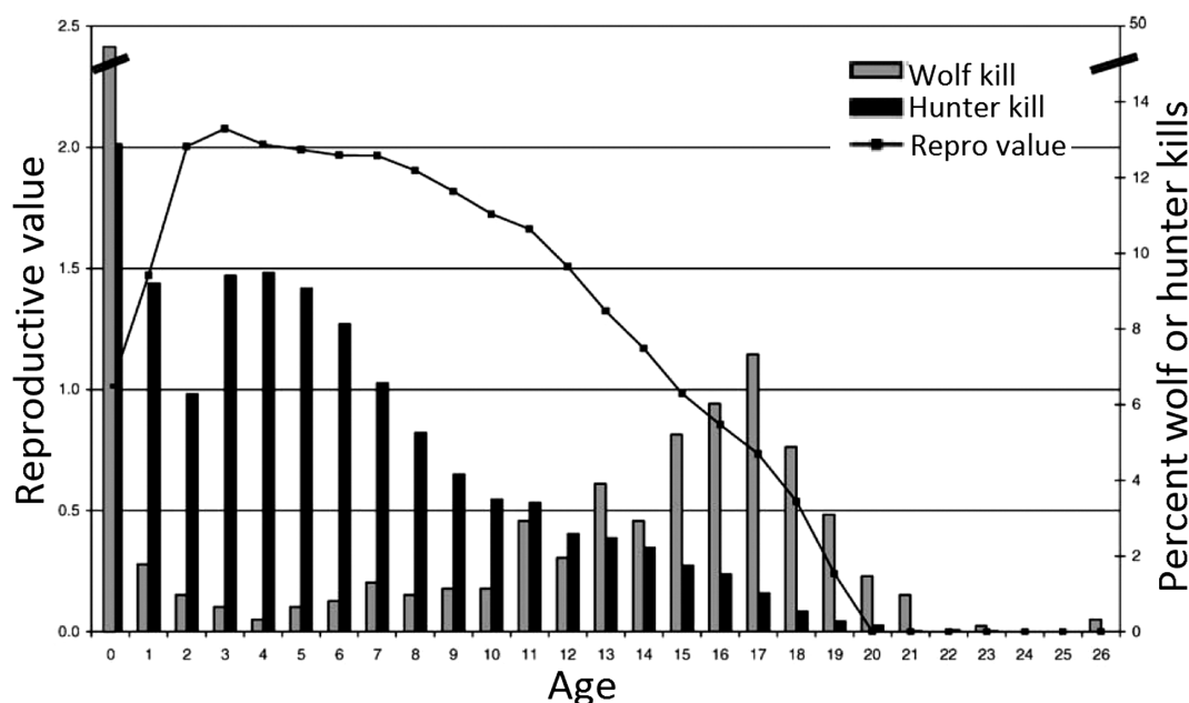
Fig. 3. —Age distributions of female elk ( Cervus elaphus ) killed by hunters versus wolves ( Canis lupus ), 1995–2001. Elk calves killed by wolves is 49% of the total. The line is the reproductive value for females of each age class (adapted from Wright et al. 2006).
