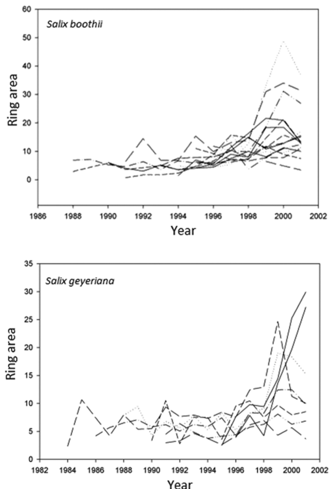
Fig. 4. —Growth by 2 species of willow, Salix boothii and S. geyeriana , before and after wolf ( Canis lupus ) reintroduction in 1995 measured by dendrochronology (Beyer et al. 2007). Each line is a separate sampling site illustrating substantial variation in the response of willows to wolf recovery. Courtesy of H. Beyer.
