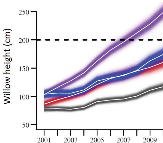
Fig. 5. —Height response of willows ( Salix spp.) to 4 replicated treatments of herbivory using exclusion fences to eliminate grazing and dams to simulate beaver ( Castor canadensis ) dams. White lines are mean response with shading of 95% prediction intervals for controls in gray, unbrowsed in red, dammed in blue, and both grazing exclusion and dammed in purple. Dashed line at 200 cm is height required to escape herbivory (from Marshall et al. 2013).
